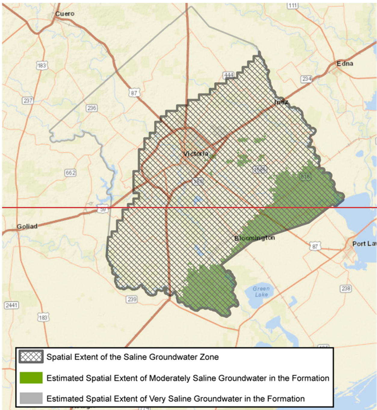
Figure 2: Goliad Saline Groundwater Zone and 5: Spatial Extent of the Moderately Saline Groundwater ExtentZone
