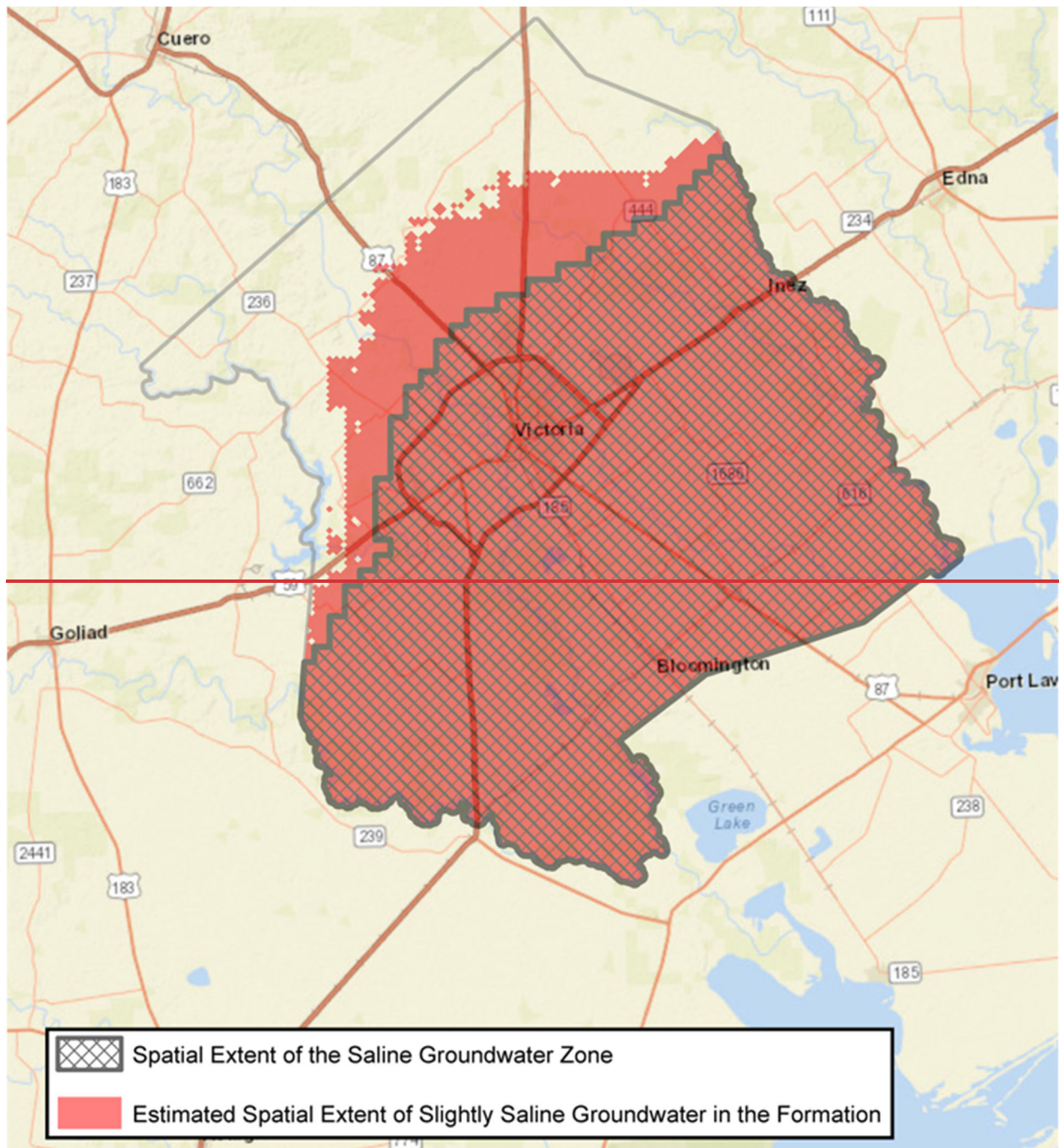
Figure 4: Spatial Extent of the Slightly Saline Groundwater Extent Zone
